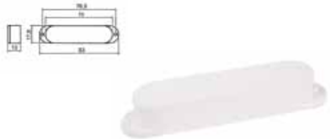
pickup cover, Stallion single coil, mat 83,0-70,0x17,8x18,0mm, no holes, 3 pcs
