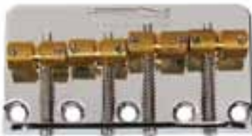
Wilkinson bridge-tailpiece JB-Pucher bass, pitch 19mm, brass saddles
