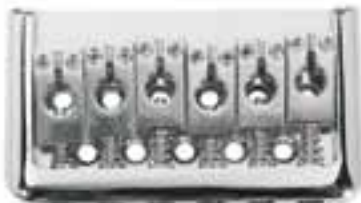
bridge-tailpiece, PRS-model, pitch 10,5mm
